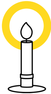
Candidate = Candle
